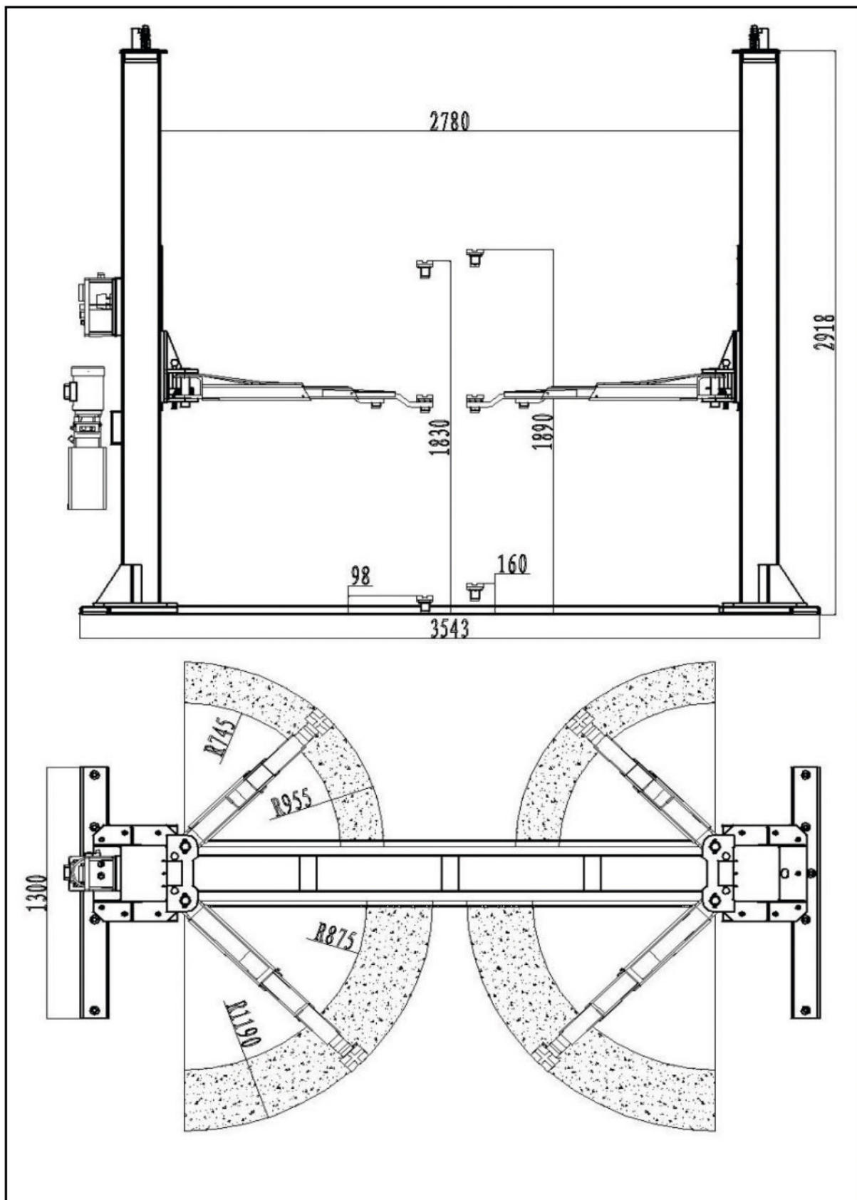
Picture 1 (lift dimension)
